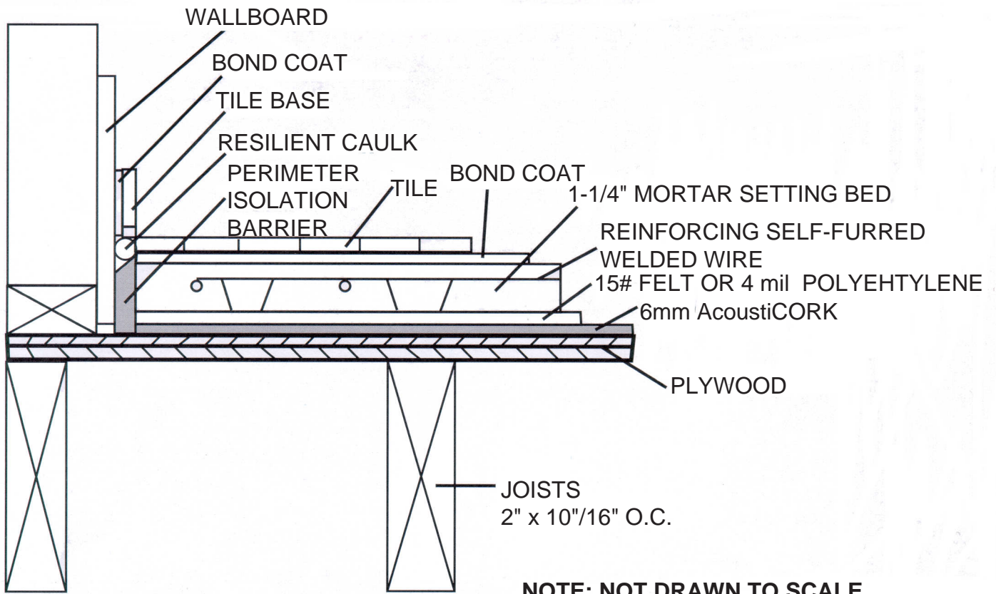
Tile Floors over 1-1/4" Mortar Setting Bed on a Wood Floor
